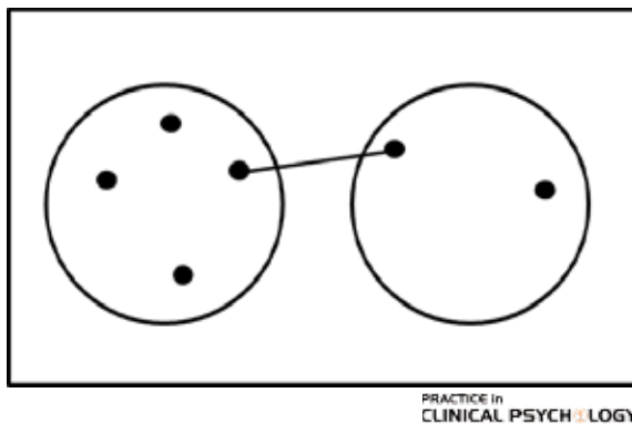
Figure 2. The single linkage procedure for calculating distance between clusters.
