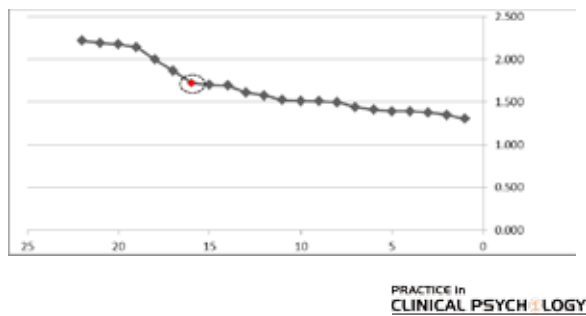
Figure 3. Line graph for coefficients of the final 22 steps of the single linkage clustering.
