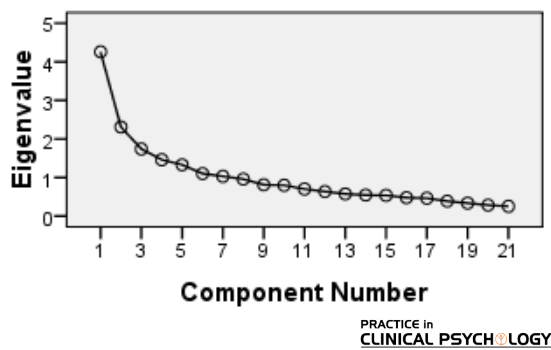
Figure 1. Eigenvalues on the scree plot of DBS.
